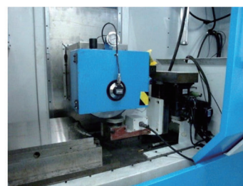
Fig.3 2-axis cup-wheel dressing equipment
